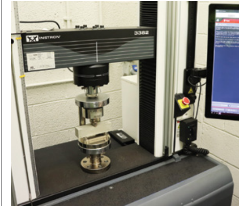
Flexural Test
