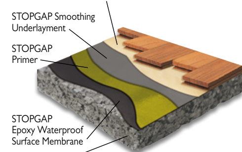
Subfloor
